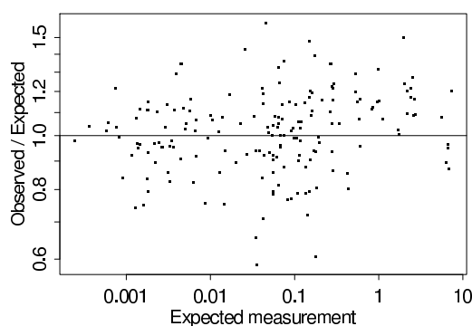
Figure 19.9 Observed PERC concentrations (for all individuals in the study) divided by expected concentrations, plotted vs. expected concentrations. The x and y-axes are on different (logarithmic) scales: observations vary by a factor of 10,000, but the relative errors are mostly between 0.8 and 1.25. Because the expected concentrations are computed based on a random draw of the parameters from their posterior distribution, the figure shows the actual misfit estimated by the model, without the need to adjust for fitting.
