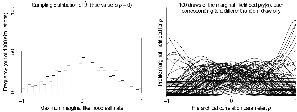
Figure 13.4 From a simulated varying-intercept, varying-slope hierarchical regression with identity group-level covariance matrix: (a) Sampling distribution of the maximum marginal likelihood estimate \hat{\rho} of the group-level correlation parameter, based on 1000 simulations of data from the model. (b) 100 simulations of the marginal profile likelihood, L_{\text{profile}}(\rho|y) = \max_{\tau_1, \tau_2} p(y|\tau_1, \tau_2, \rho) . In this example, the maximum marginal likelihood estimate is extremely variable and the likelihood function is not very informative about \rho . (In some cases, the profile likelihood for \rho is flat in some places; this occurs when the corresponding estimate of one of the variance parameters ( \tau_1 or \tau_2 ) is zero, in which case \rho is not identified.)
