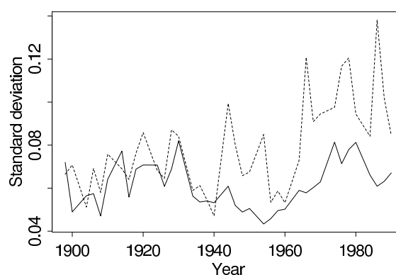
Figure 14.4 Posterior medians of standard deviations \sigma_1 and \sigma_2 for elections with incumbents (solid line) and open-seat elections (dotted line), 1898–1990, estimated from the model with two variance components. (These years are slightly different from those in Figure 14.2 because this model was fit to a slightly different dataset.)
