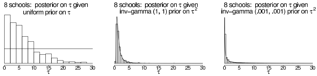
Figure 5.9 Histograms of posterior simulations of the between-school standard deviation, \tau , from models with three different prior distributions: (a) uniform prior distribution on \tau , (b) inverse-gamma(1, 1) prior distribution on \tau^2 , (c) inverse-gamma(0.001, 0.001) prior distribution on \tau^2 . Overlain on each is the corresponding prior density function for \tau . (For models (b) and (c), the density for \tau is calculated using the gamma density function multiplied by the Jacobian of the 1/\tau^2 transformation.) In models (b) and (c), posterior inferences are strongly constrained by the prior distribution.
